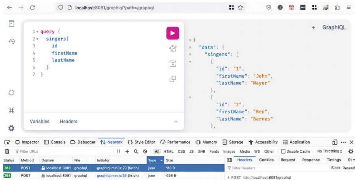
Figure 16-10 GraphiQL web console with a simple query
