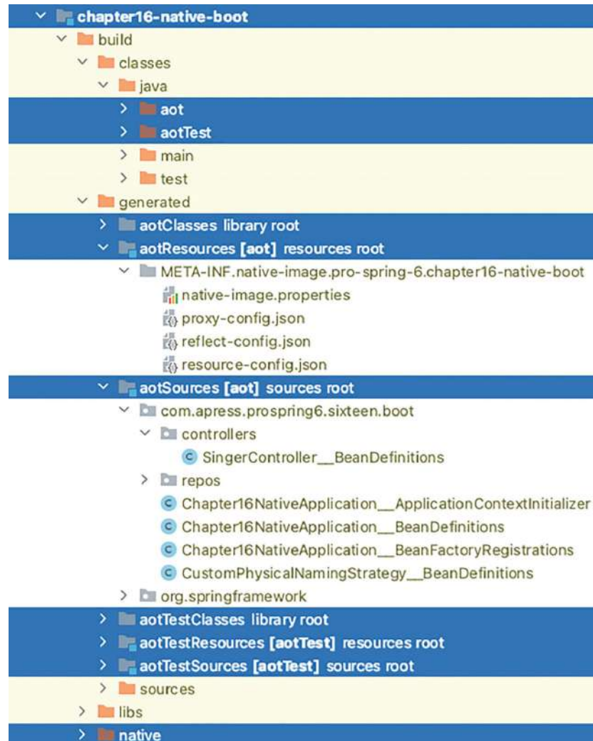
Figure 16-3 Intermediary files created by the build process that produces a native image
