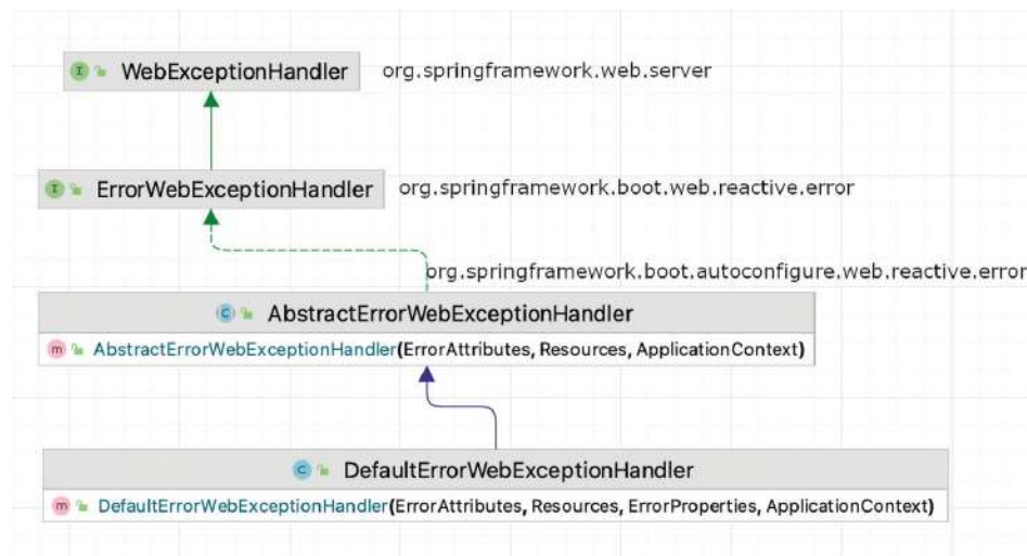
Figure 20-5 WebExceptionHandler hierarchy
