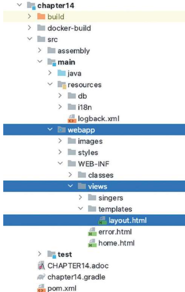
Figure 14-6 The internal structure of chapter -14 project
