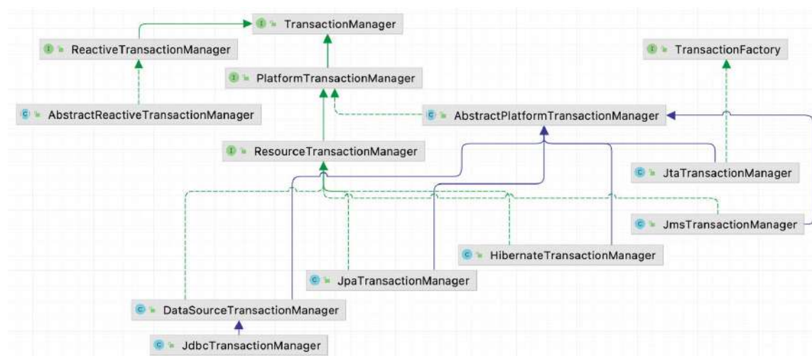
Figure 9-2 PlatformTransactionManager implementations
