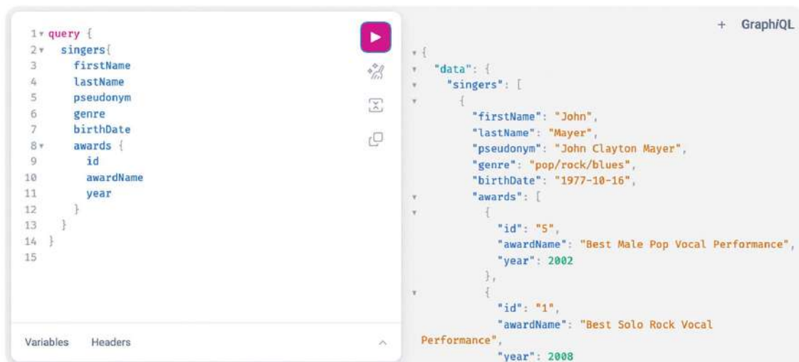
Figure 16-11 GraphiQL web console with a nested query
