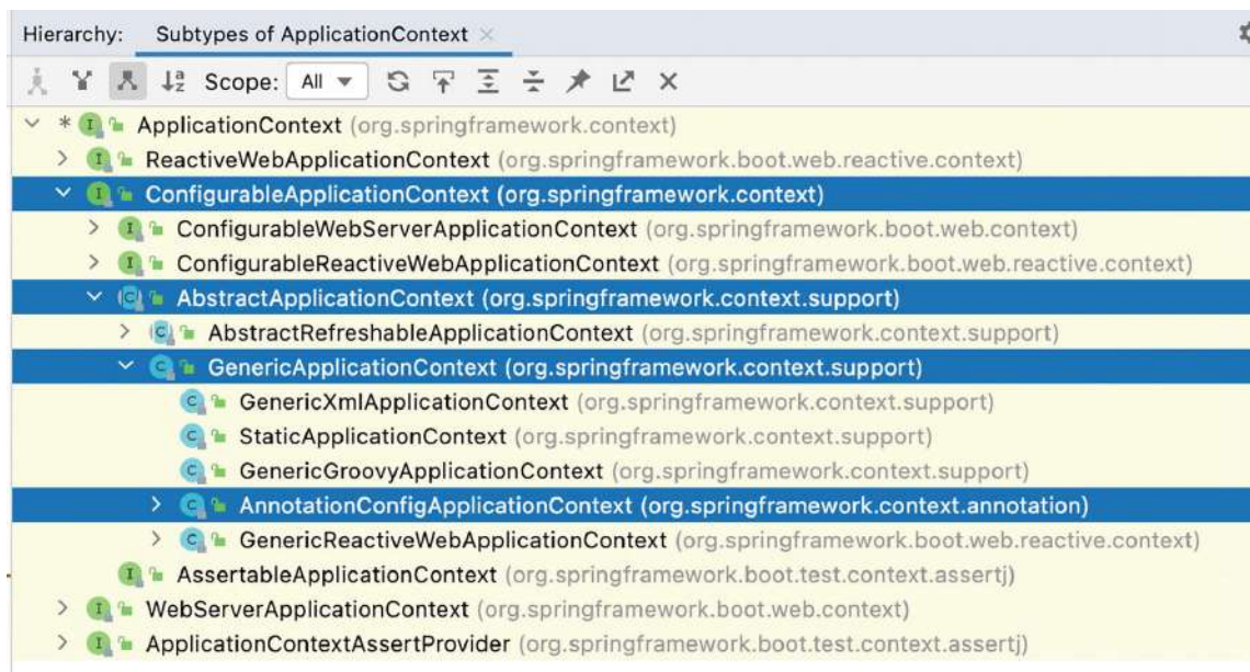
Figure 3-5 AnnotationConfigApplicationContext hierarchy
