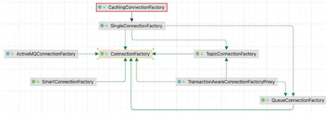
Figure 13-5 jakarta.jms.ConnectionFactory hierarchy
