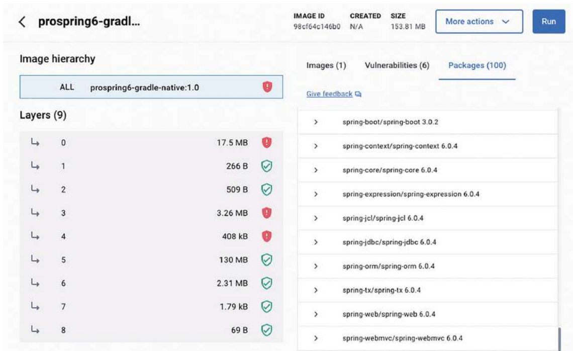
Figure 16-5 Docker dashboard showing the details of the prospring6-gradle-native:1.0 image
