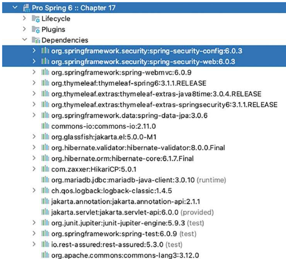
Figure 17-1 Project chapter17 dependencies
