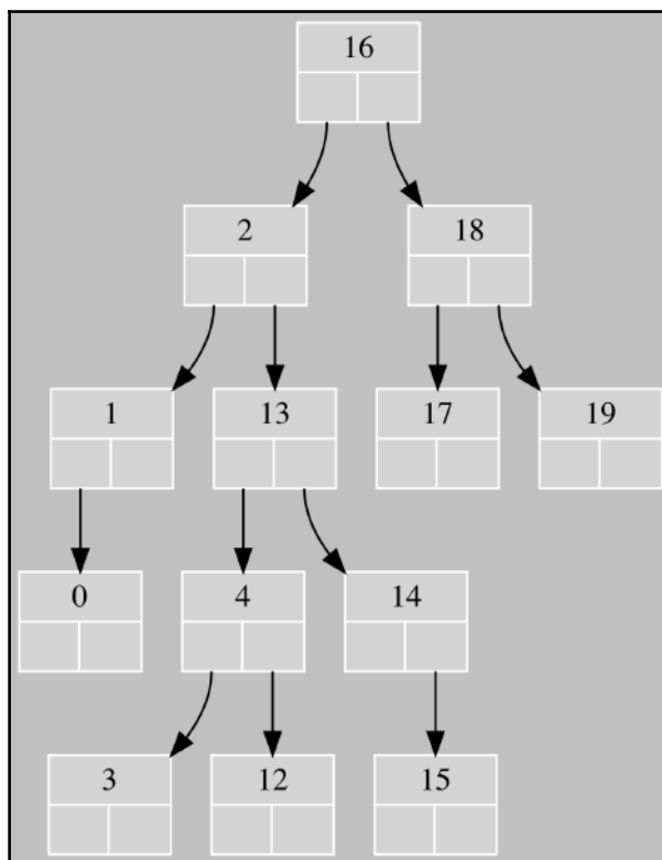
A binary tree
