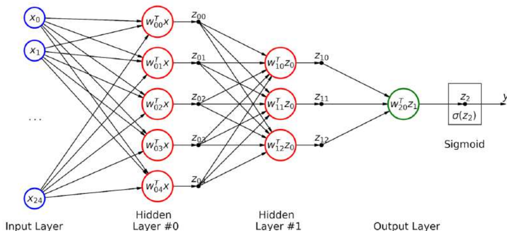
Figure 4.6 - Deep-ish model
