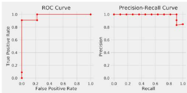
Figure 3.18 - Scikit-Learn's curves
