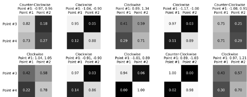
Figure 9.20 - Attention scores
