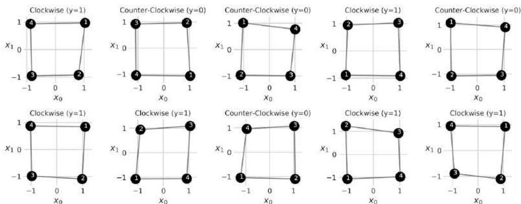
Figure 8.4 - Sequence dataset
