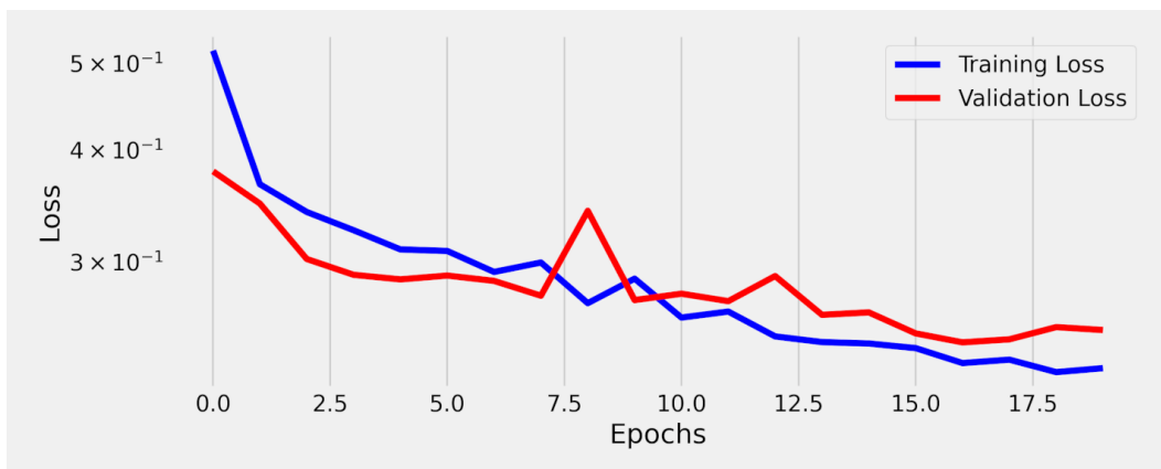
Figure 11.19 - Losses—bag-of-embeddings (BoE)
