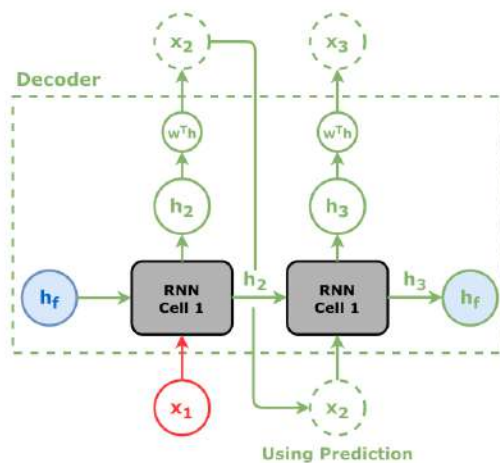
Figure 9.5 - Decoder
