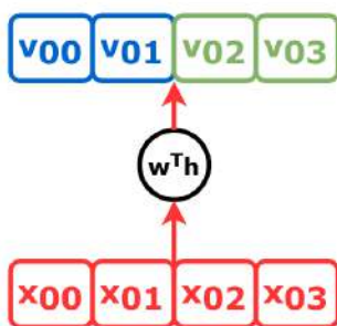
Figure 10.1 - Narrow attention
