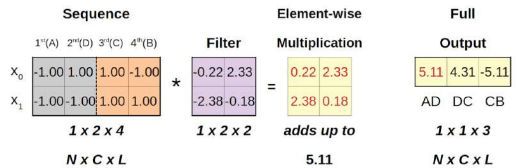
Figure 8.34 - Applying filter over the “perfect” square
