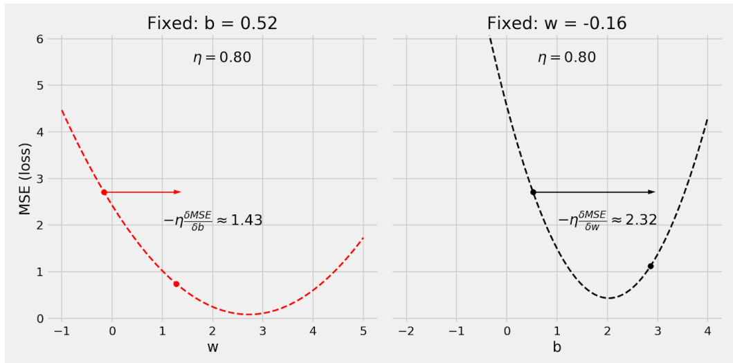
Figure 0.11 - Using a high learning rate
