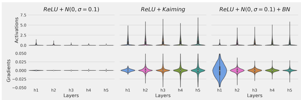
Figure E.3 - The effect of batch normalization
