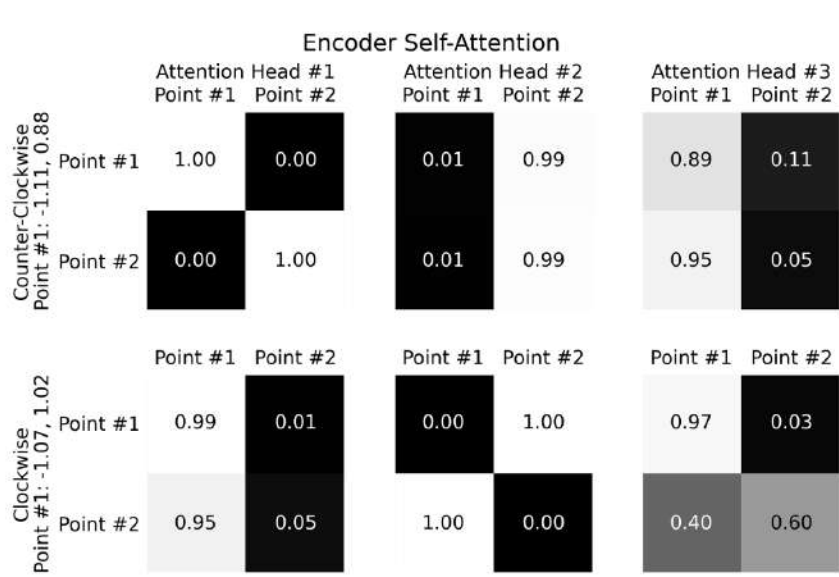
Figure 9.51 - Encoder’s self-attention scores for its three heads
