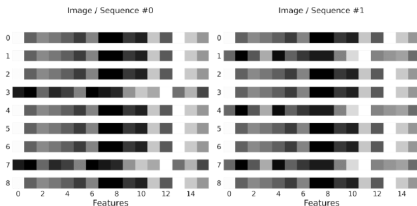
Figure 10.26 - Two patch embeddings
