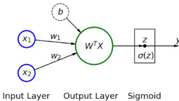
Figure 3.5 - The (second) simplest of all neural networks
