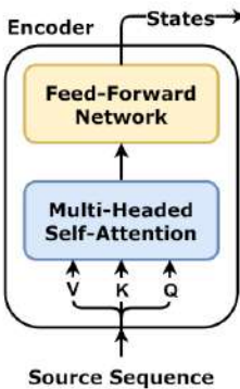
Figure 9.26 - Encoder with self-attention (diagram)
