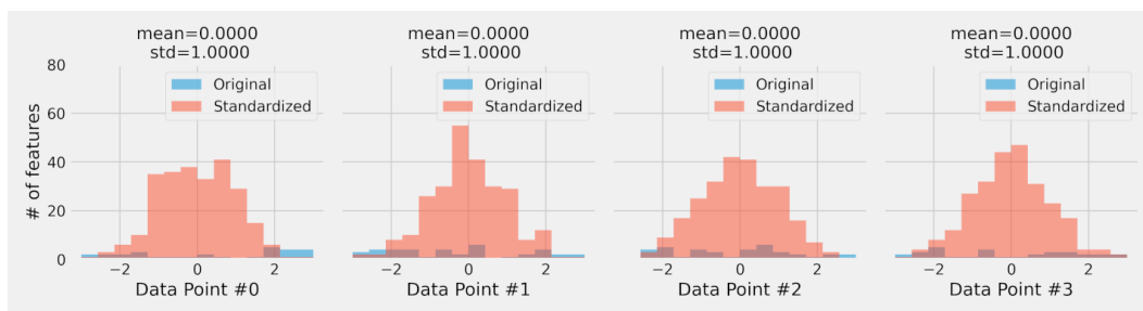
Figure 10.12 - Distribution of layer-normalized feature values
