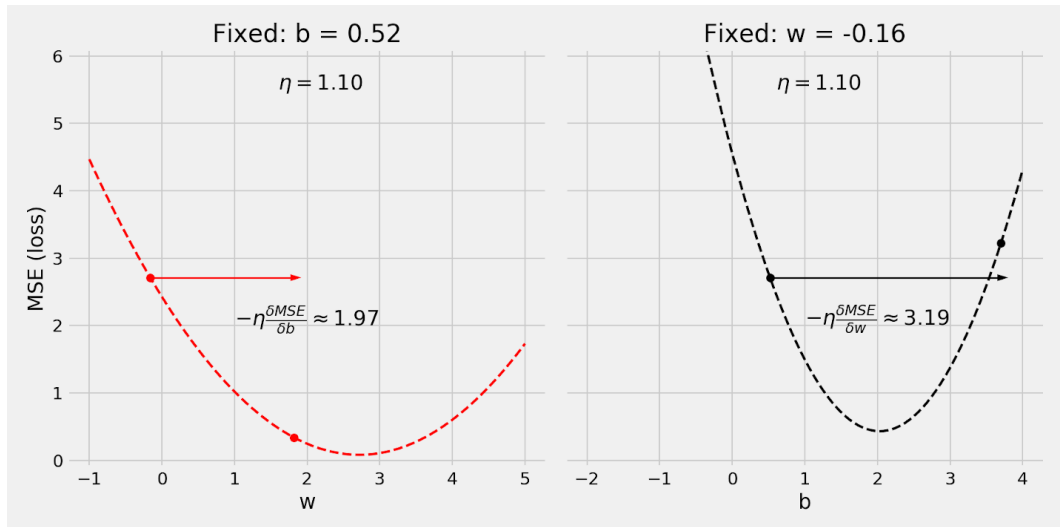
Figure 0.12 - Using a really high learning rate
