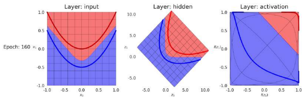
Figure B.7 - Activated feature space—TanH
