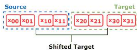
Figure 9.31 - Shifted target sequence
