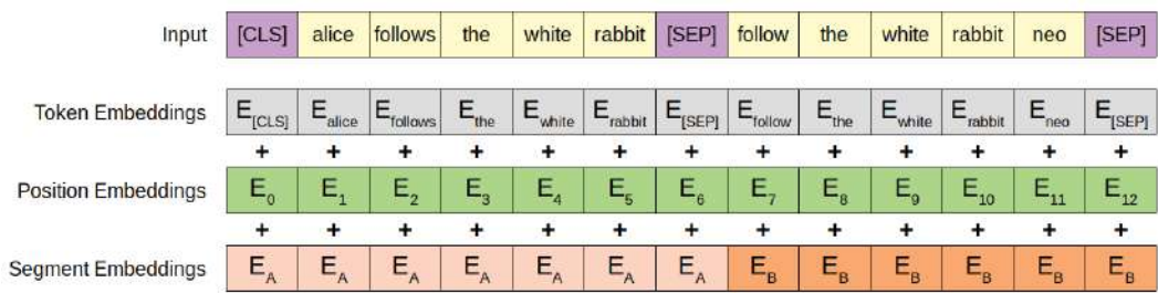
Figure 11.25 - BERT's input embeddings
