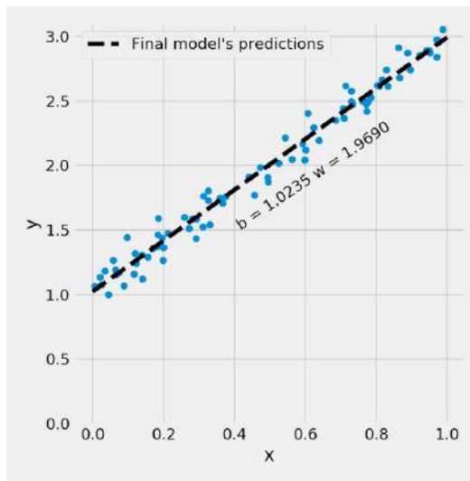
Figure 0.18 - Final model's predictions
