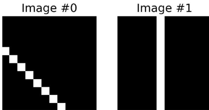
Figure 10.25 - Two images
