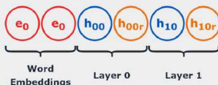
Figure 11.23 - ELMo embeddings
