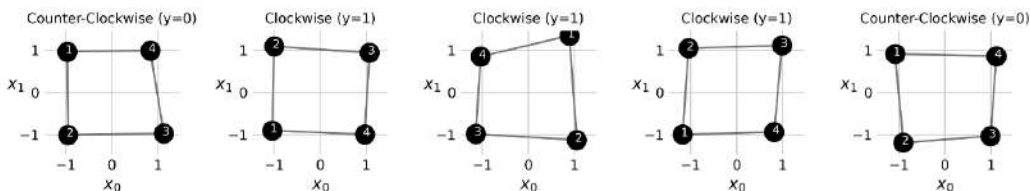
Figure 9.3 - Sequence dataset
