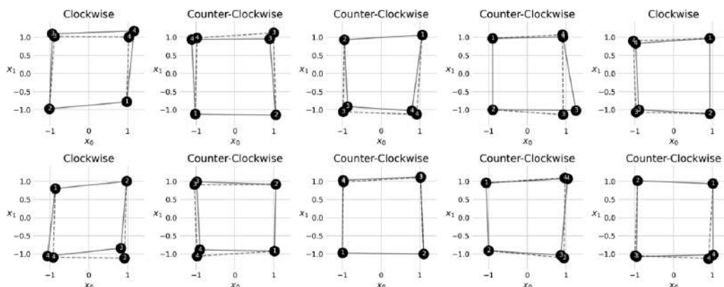
Figure 10.19 - Predictions
