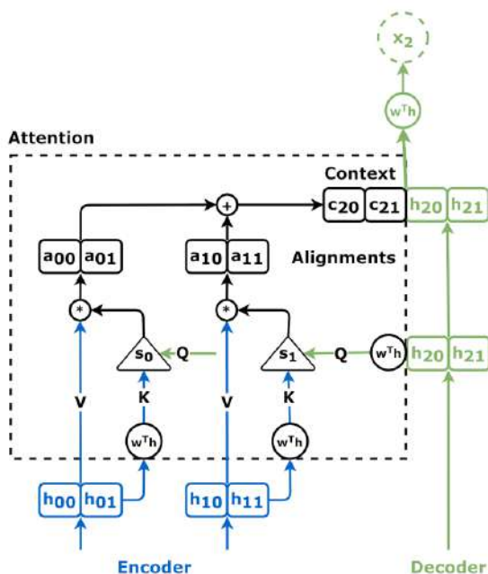
Figure 9.16 - Attention mechanism
