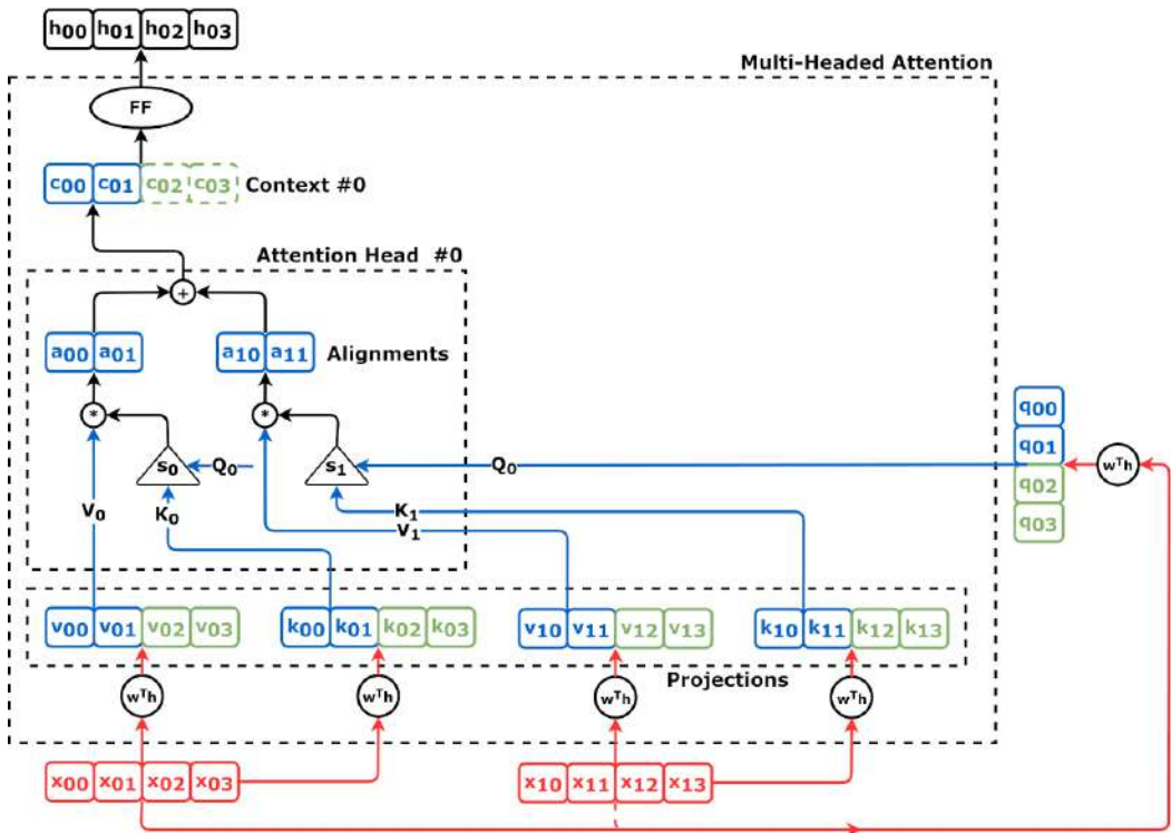
Figure 10.3 - Self-(narrow)attention mechanism
