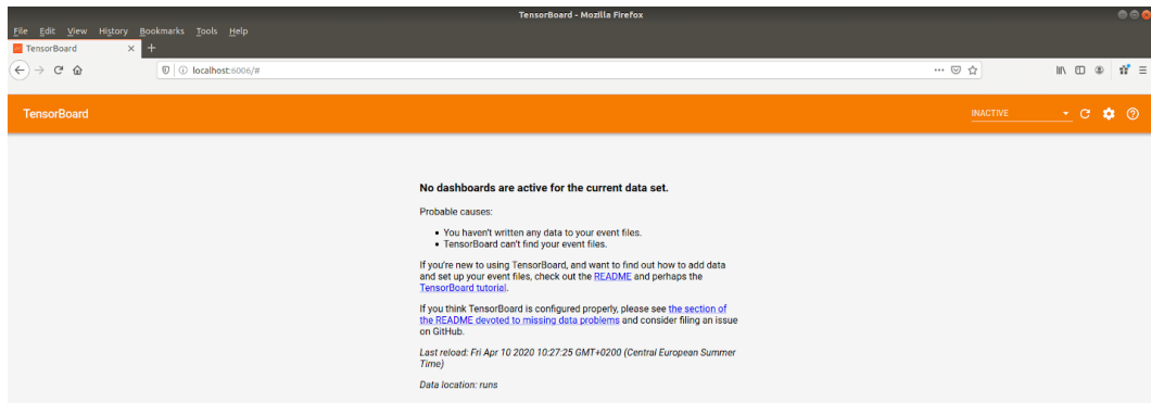
Figure 2.3 - Empty TensorBoard
