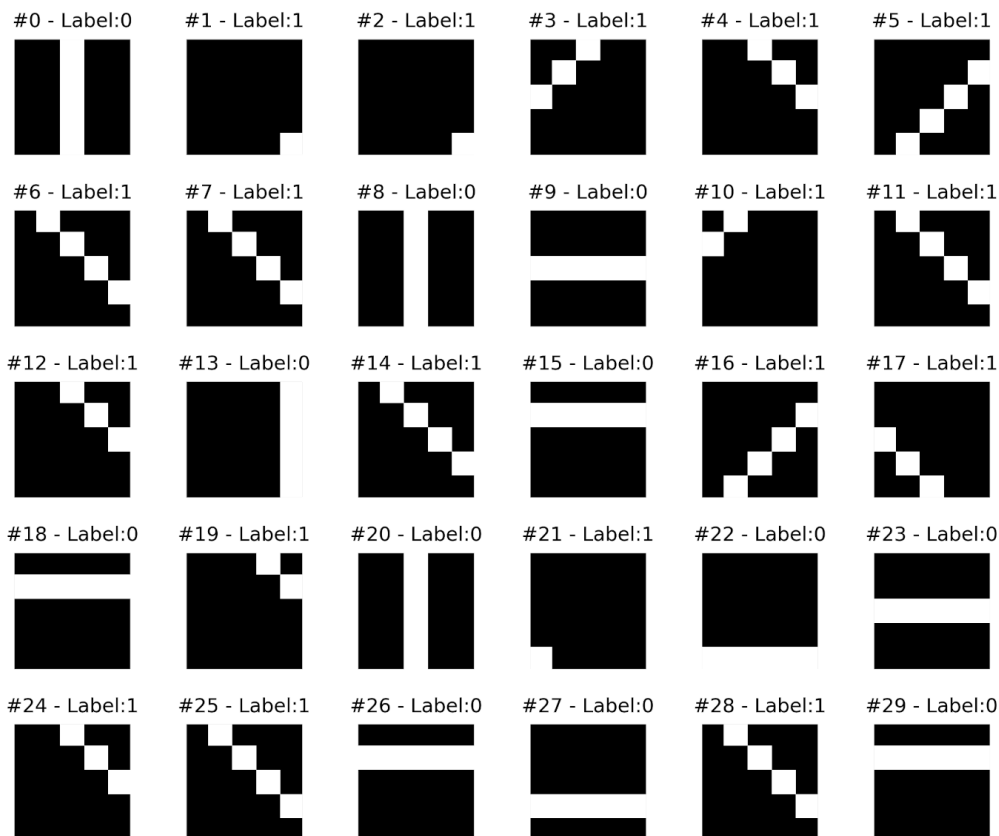
Figure 4.1 - Image dataset
