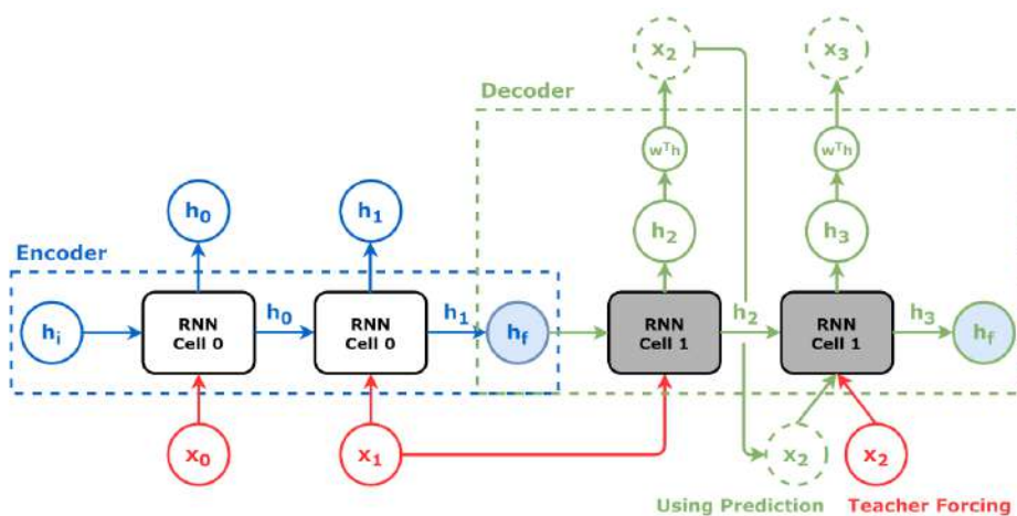
Figure 9.6 - Encoder + decoder
