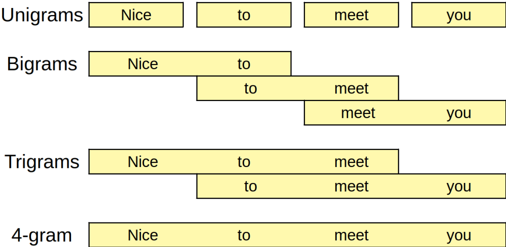
Figure 11.8 - N-grams
