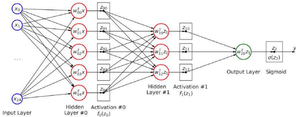
Figure 4.16 - Deep model (for real)
