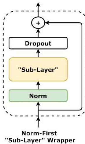
Figure 10.31 - "Sub-Layer" wrapper—norm-first
