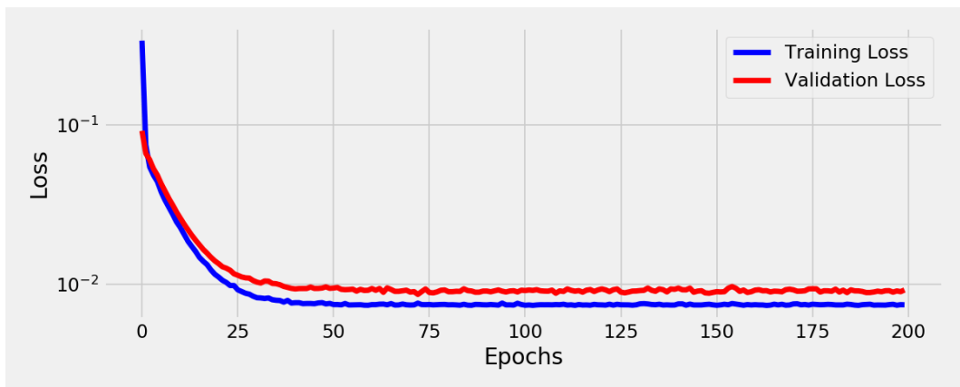
Figure 2.1.2 - Losses
