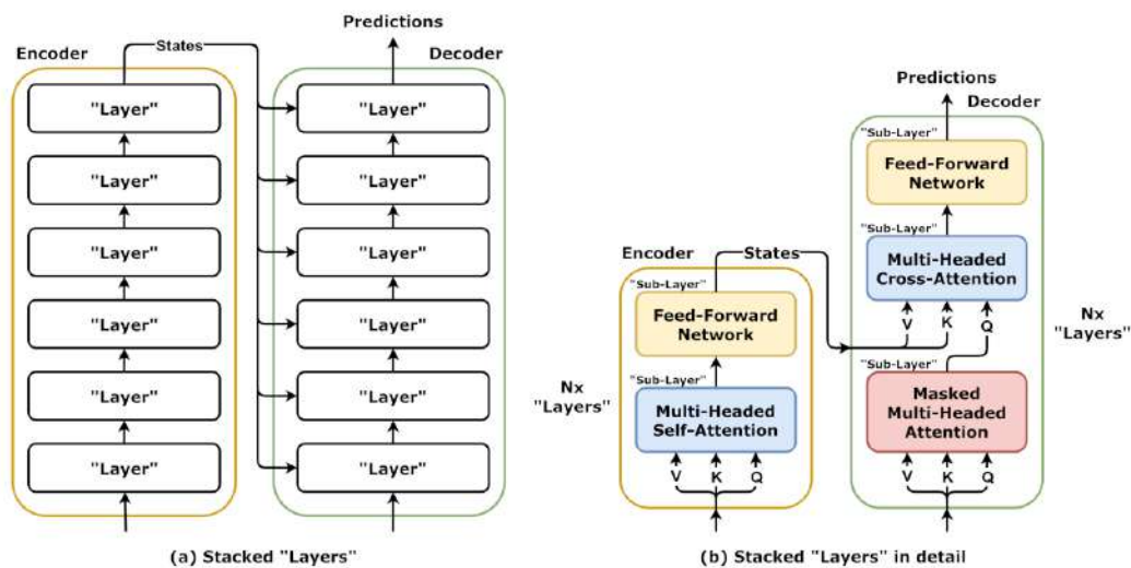
Figure 10.6 - Stacked "layers"
