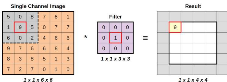
Figure 5.3 - Shrinking images with convolutions
