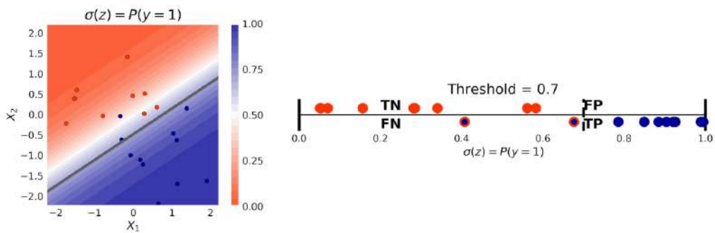
Figure 3.15 - Using a high threshold
