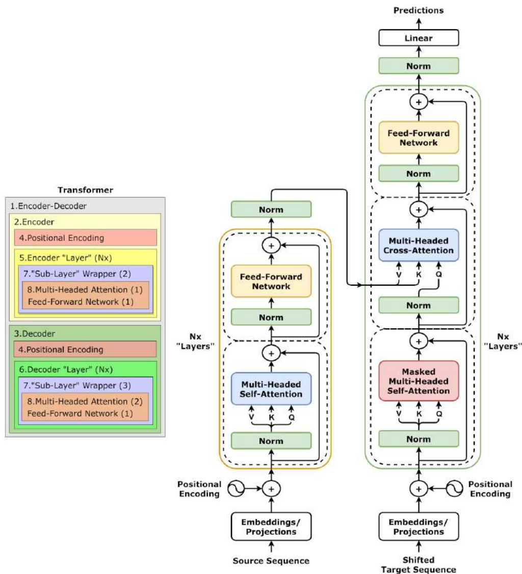
Figure 10.30 - The Transformer
