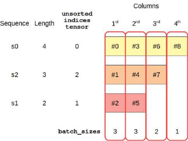
Figure 8.27 - Packing sequences
