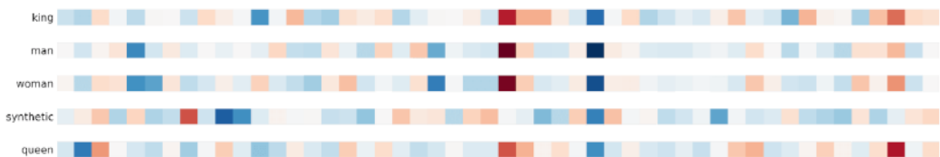
Figure 11.17 - Synthetic queen
