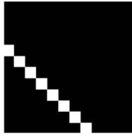
Figure 10.20 - Sample image—label "2"
