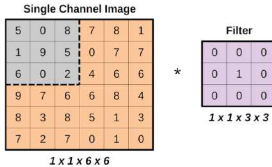
Figure 5.1 - Identity filter
