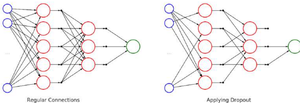
Figure 6.6 - Applying dropout
