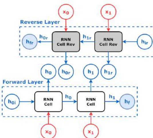
Figure 8.11 - Bidirectional RNN
