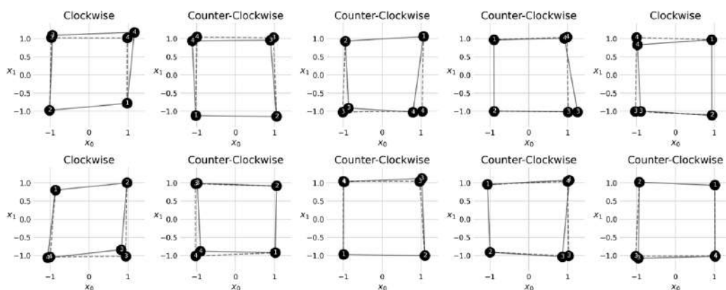
Figure 10.16 - Predictions
