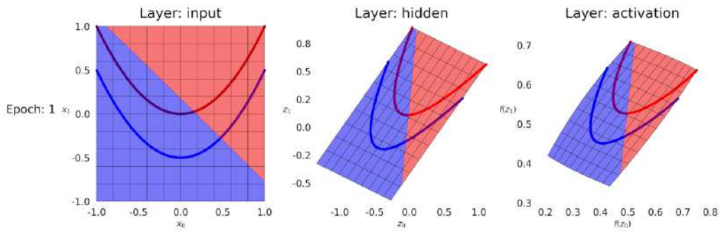
Figure B.5 - In the beginning...
