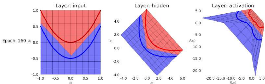
Figure B.9 - Activated feature space—PReLU
